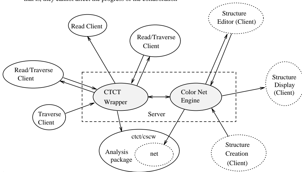
Figure 8: System architecture of a Trellis implementation.
